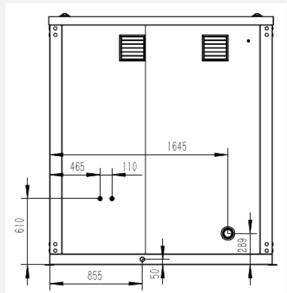
External elevation B
