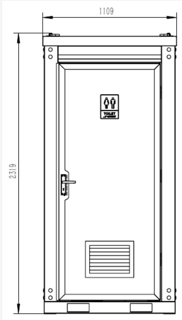
External elevation A
