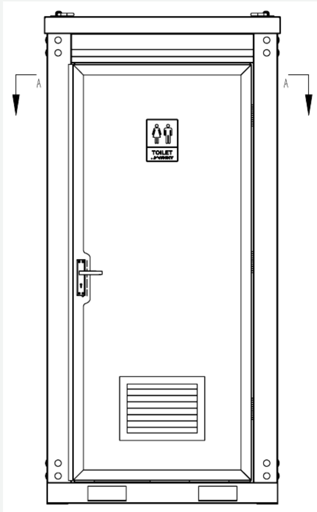
Front elevation
