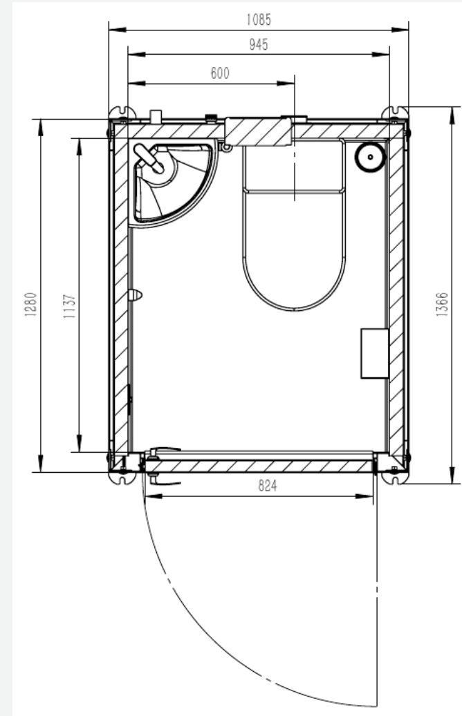
Bird's-eye plan
