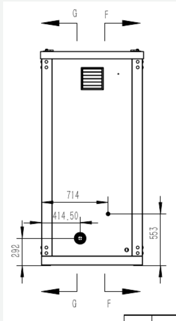
Lower section 2
