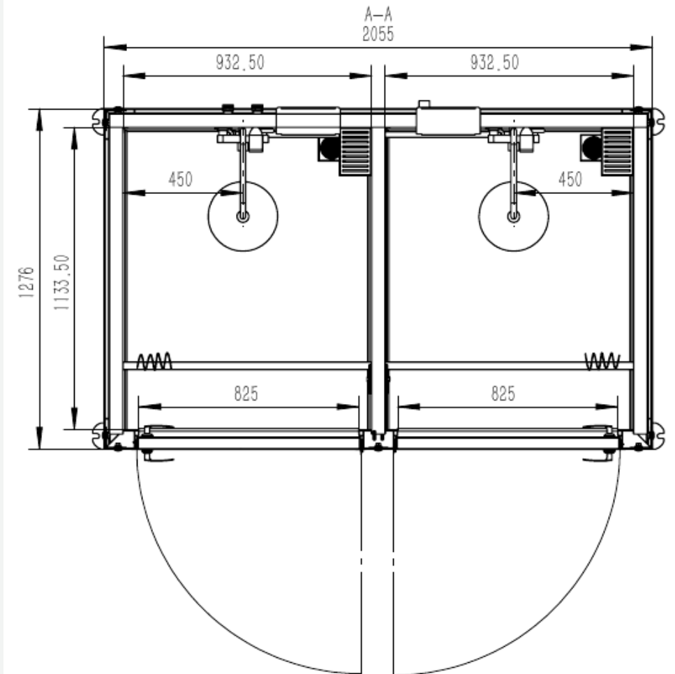
Bird's-eye plan
