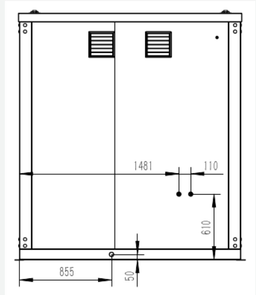
External elevation B
