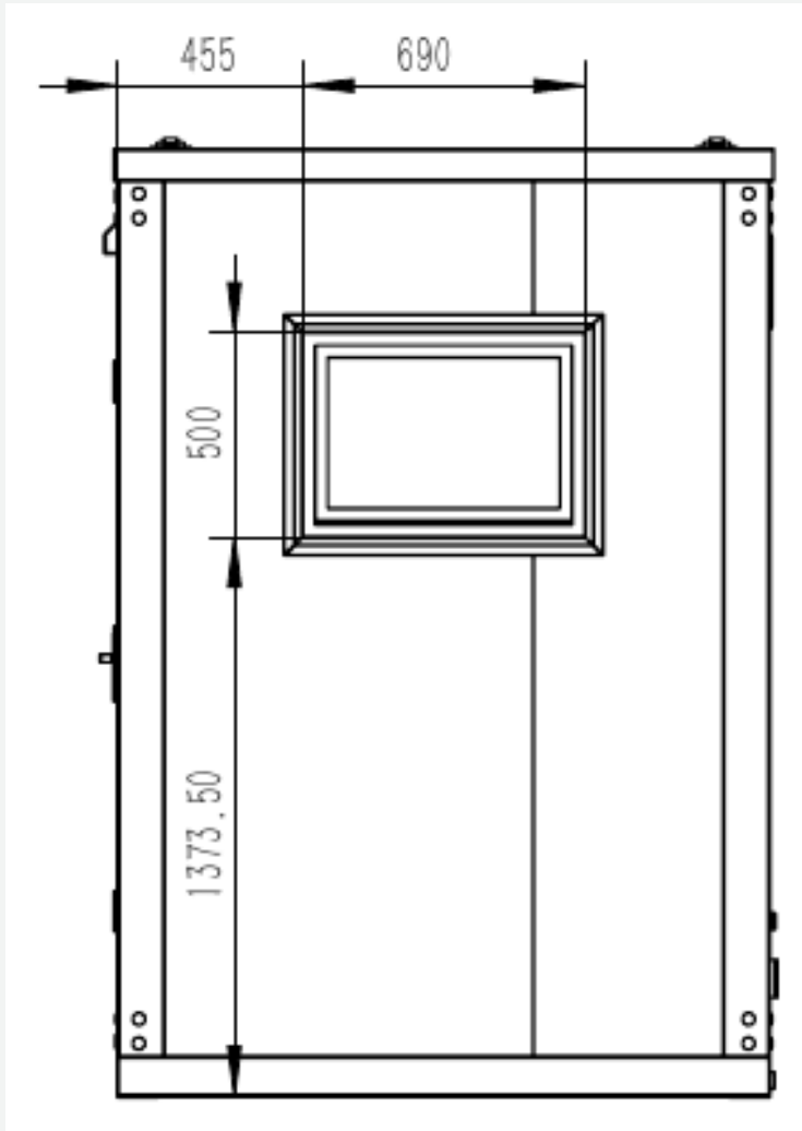
External elevation C
