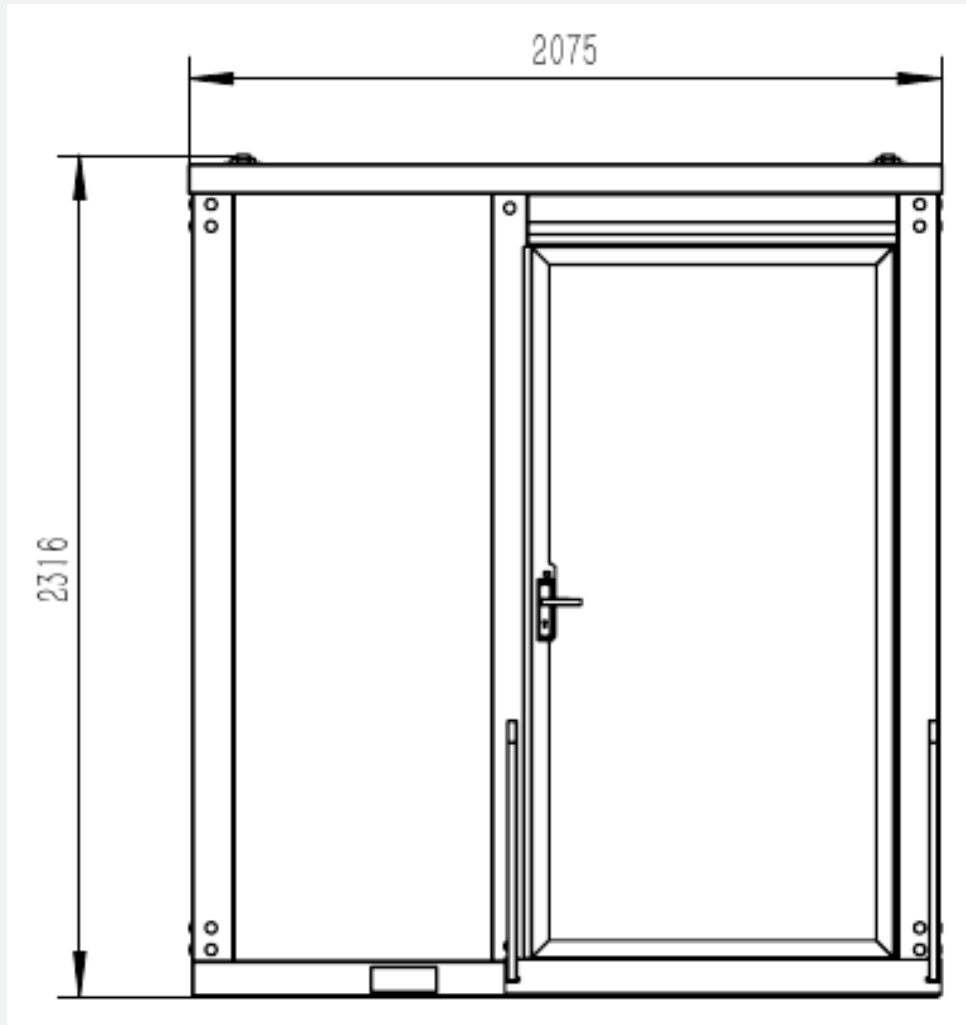
External elevation A
