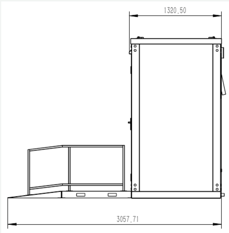
External elevation C
