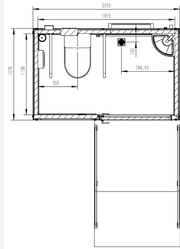
Bird's-eye plan
