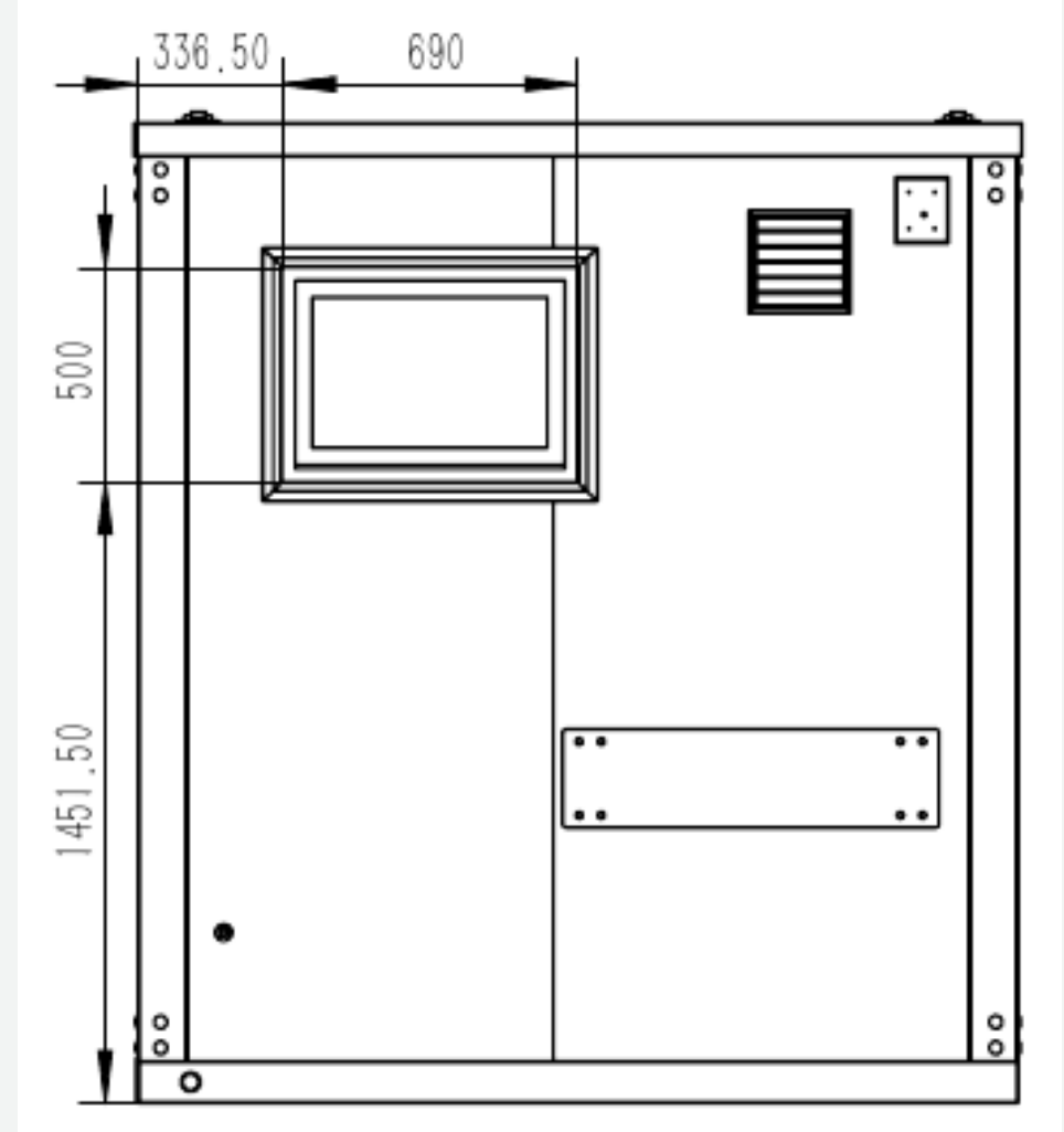
External elevation B
